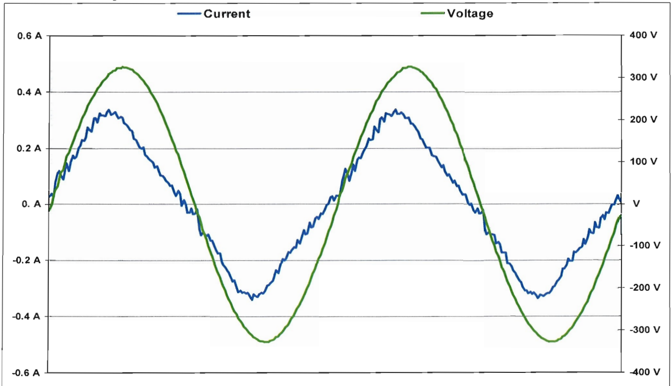
Graphics harmonics
